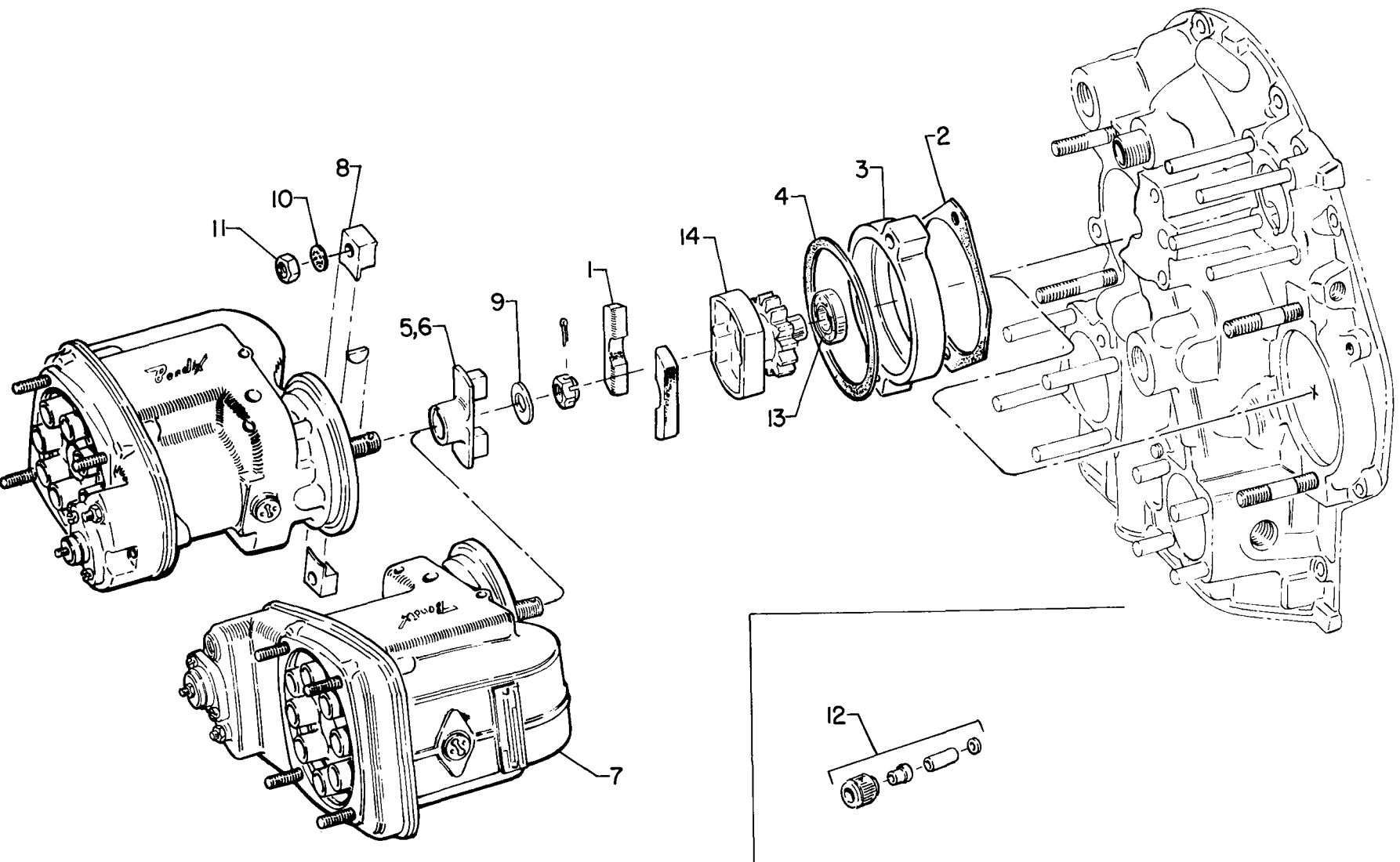
Figure 20 - Magneto Drives and Magnetos 4-2
