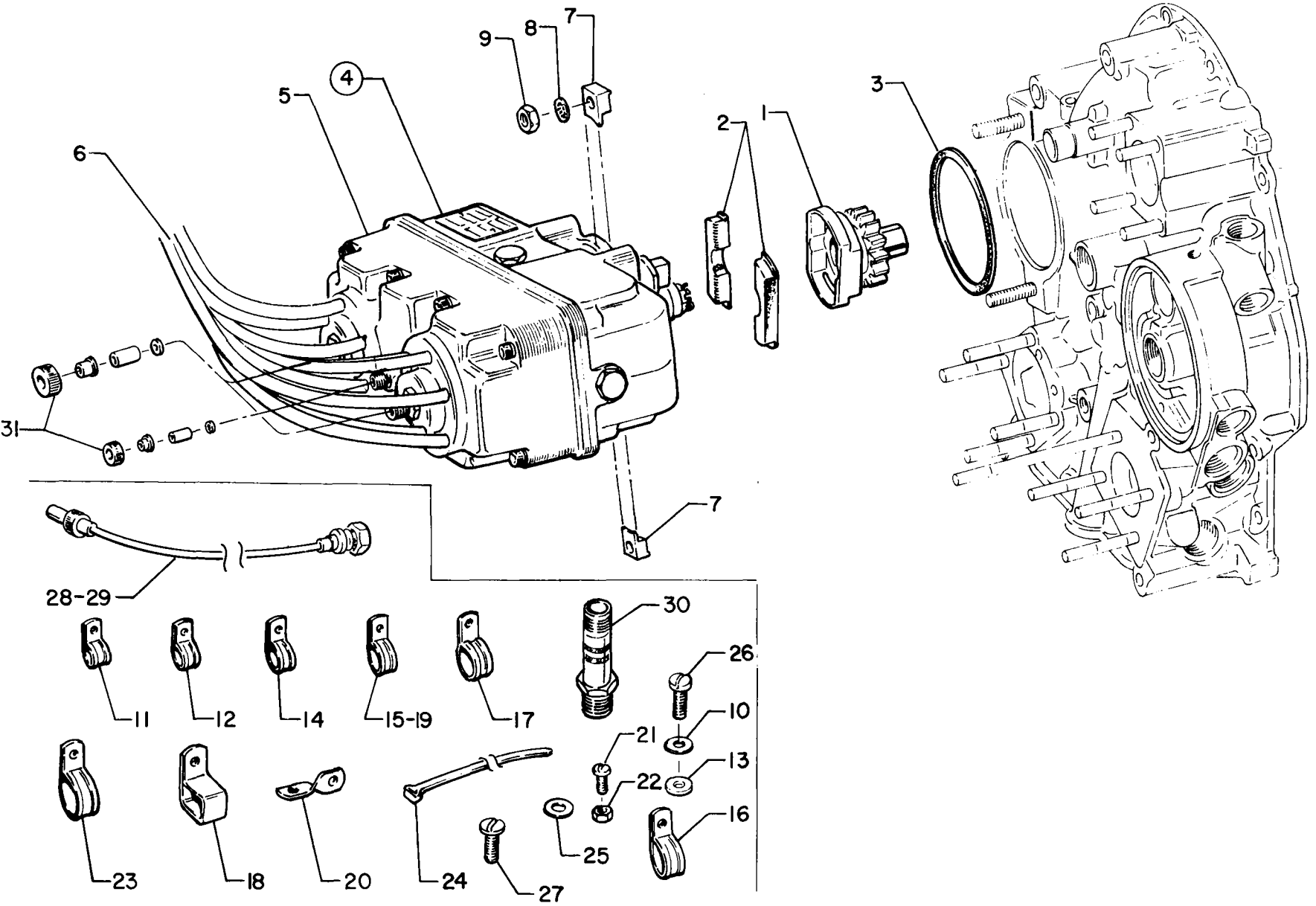
Figure 21 - Magneto Drives, Magnetos, Lead Assemblies and Spark Plugs (Dual Magnetos) 44
