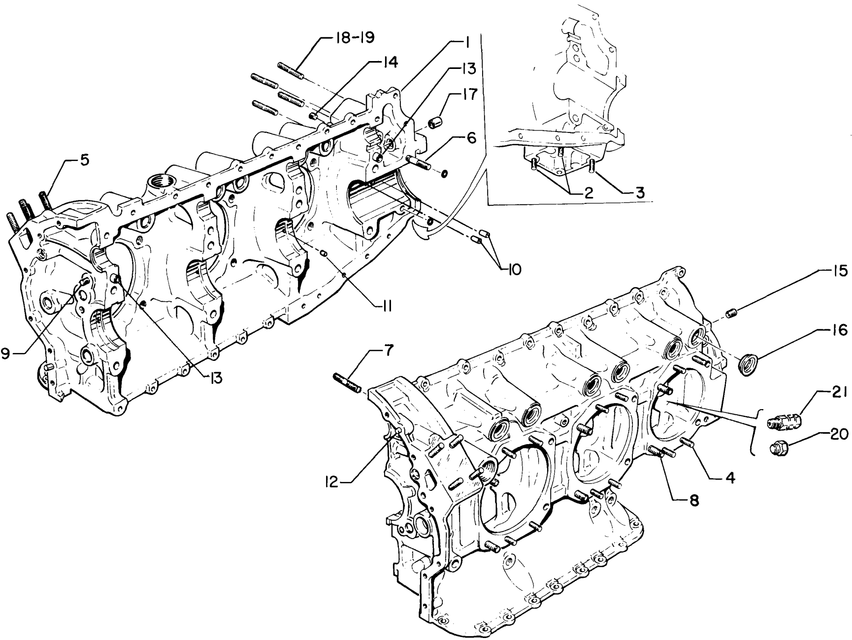
Figure 1 - Crankcase Assembly
