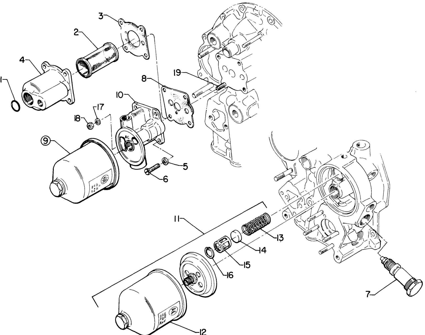
Figure 14 - Oil Pressure Screen, Filter and Oil Cooler Bypass Valve
